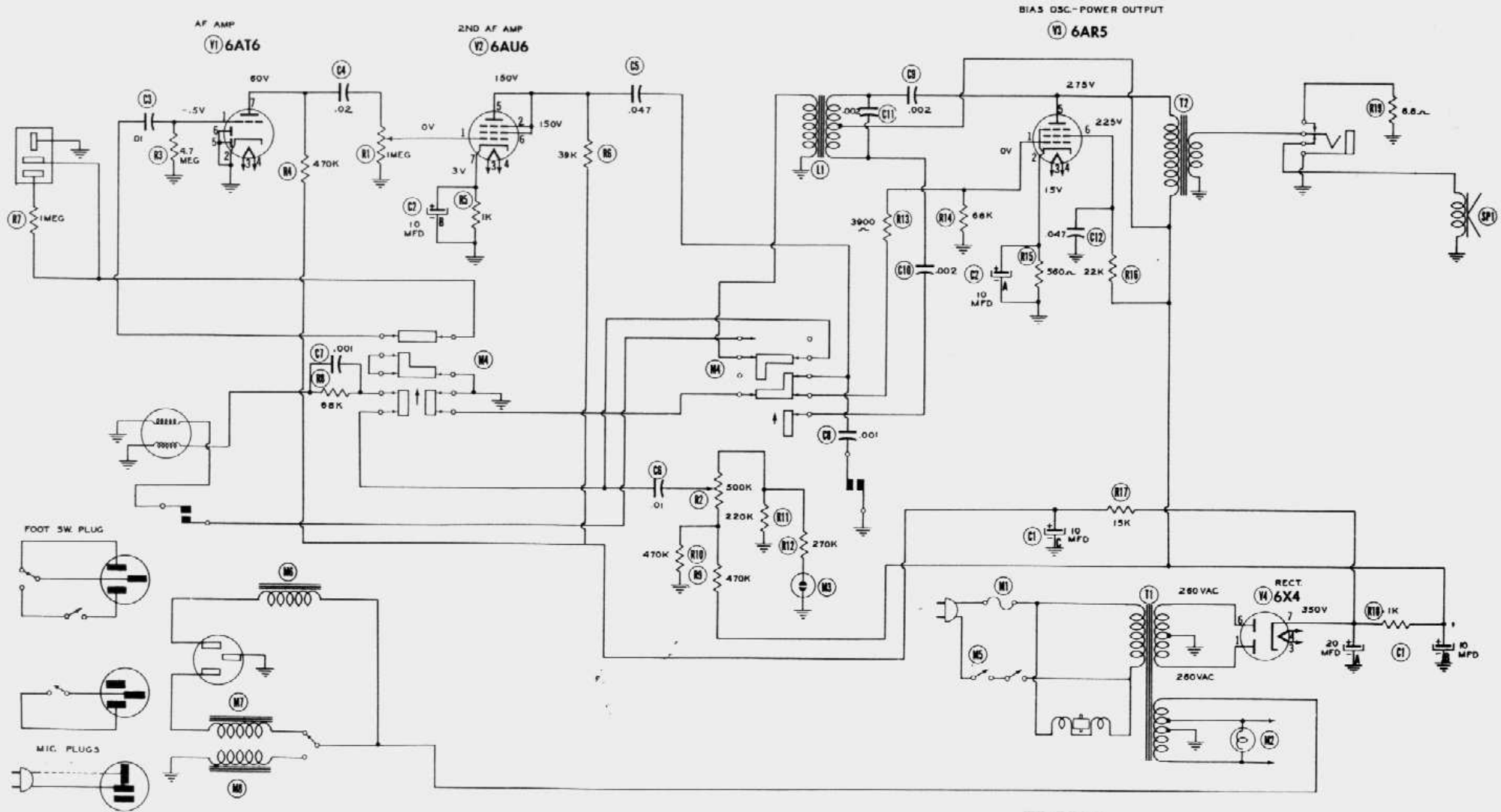
A PHOTOFAC STANDARD NOTATION SCHEMATIC
